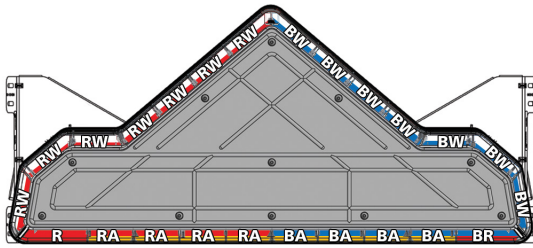
VALR44J-P1BH HOOK MOUNT
